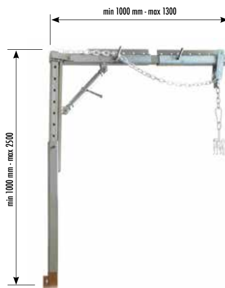
Art. 07700400 | Kit tiro verticale standard (fornito senza catena di tiro e manina) Kit vertical pull (supplied without pull chain and hooks claw)
